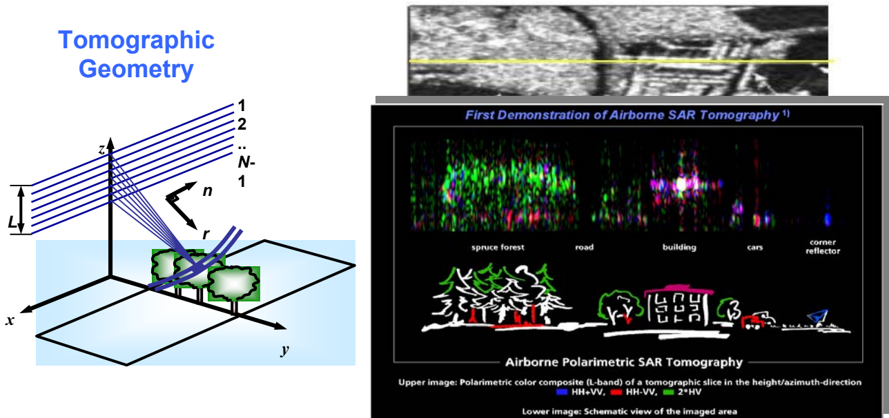
Fig. 5, Scheme and result of SAR Tomography. Left: Multi baseline imaging geometry with Synthetic Apertures in azimuth (flight path x -direction) and height (z-direction). Right: Middle image: Polarimetric color composite in the Pauli basis of a tomographic slice taken from a cut along the yellow line in the SAR image in the upper part in the height/azimuth-direction, (blue = HH + VV, red = HH - VV, green HV+VH). Lower image: Schematic representation of the imaged area. (Reigber, Moreira 2000) This image will be used and described in more detail in the Application Chapter of this Lecture Series in section 4. The polarimetric Interferometry together with some special applications will be considered and presented during the LS by Martin Hellmann.
