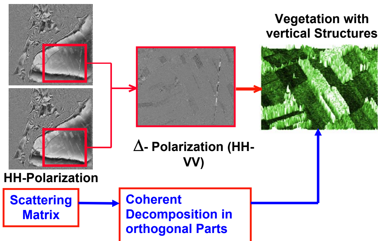
Fig.4, Example for Overlay Polarimetry with HH- and VV- Interferograms, full polarimetric one pass data take, E-SAR, L-Band, Solothurn area, Switzerland. Through the vertical vegetation (Corn) passes the horizontally polarized component mainly undisturbed down to the ground, whereas the vertical polarized part is reflected on top. In principle, the vegetation layer acts as a Polarization Filter.
