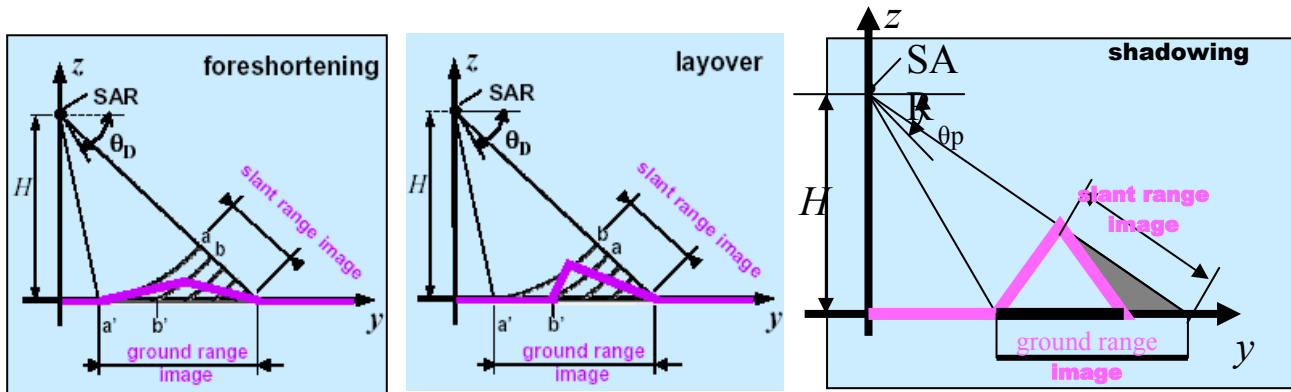
Fig. 2, Geometric Distortions in SAR Images; foreshortening: slope of local terrain is less than incidence angle leading to layover for steep terrain: slope of local terrain is less than incidence angle also; shadowing: descending slope is less than incidence angle, SNR = 0, no signal.
